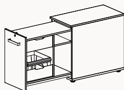
Height 740, width 430, depth 800/900/1000 mm
