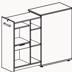
Height 1148 (3 BH), width 430, depth 800/900/1000 mm
