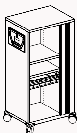
Height 1148 (3 BH), width 550, depth 436 mm
