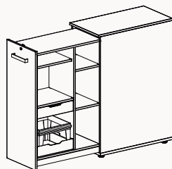
Height 1148 (3 BH), width 430, depth 800/900/1000 mm
